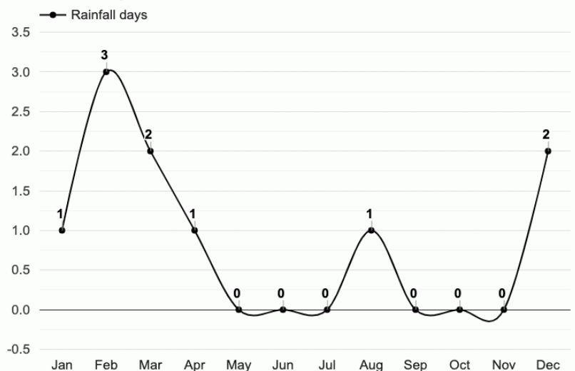
Rainfall days - Muscat, Oman
