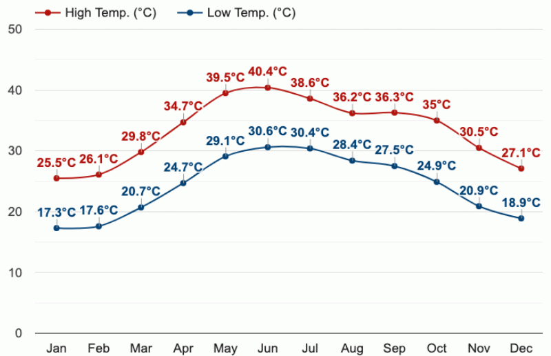
Temperature - Muscat, Oman
